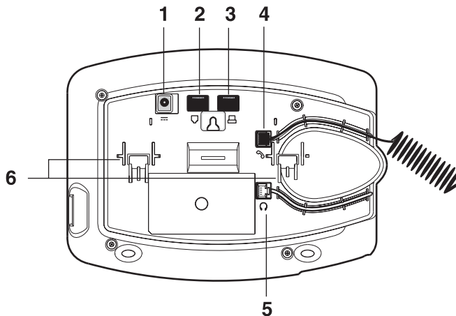
Figure 11 Underside of the 3Com 3102 Business Telephone
